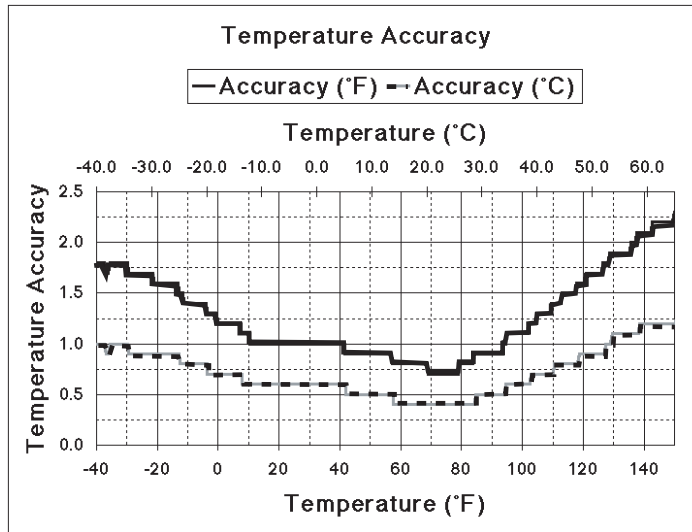
Figure 1. Temperature Accuracy
